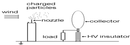
Figure 4. Type A implementation of the static wind converter system with an insulated collector. The charged particles through the charging system consisting of nozzles and electrodes .Wind transports these particles to the collector
