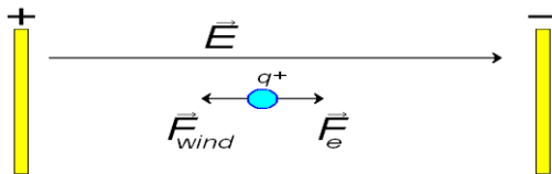
Figure 3. A positively charged particle is pushed towards the positive(+) electrode by the wind opposite to the direction of the electric field, thereby increasing the potential energy of the charged particle
